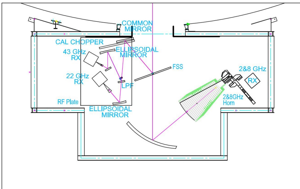
Figure 21: The KSJ quasi-optics and receiving system
